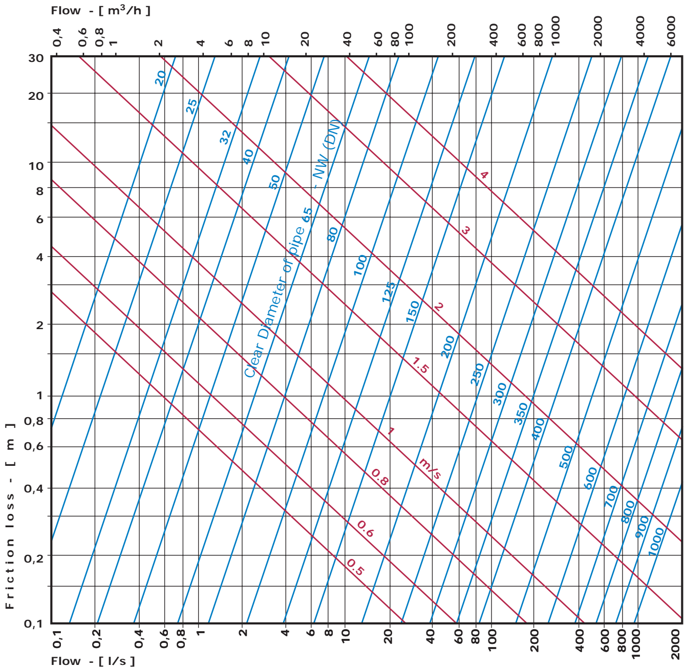
Friction loss in metres for 100m new pipeline of cast iron
