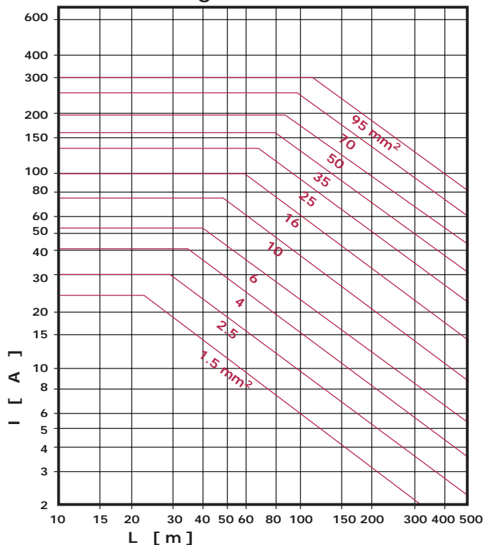
D.O.L. starting 230V multi-core cable
