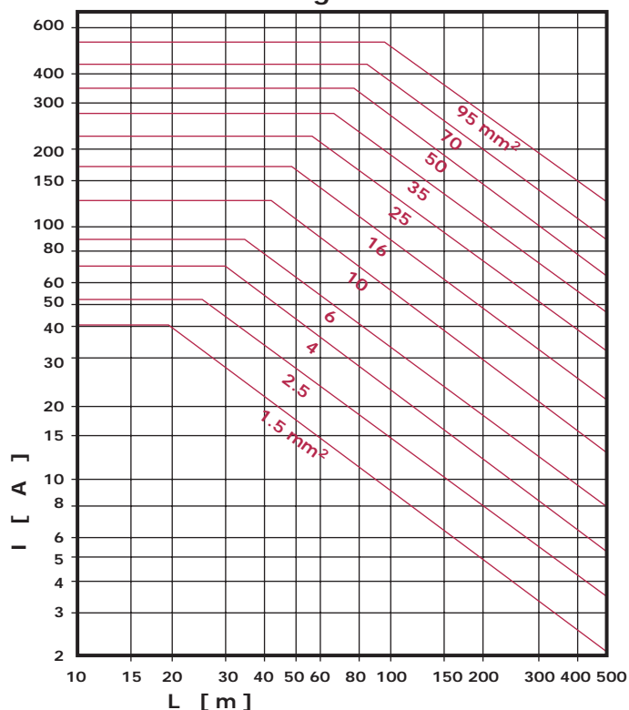
Star Delta starting 400V multi-core cable
