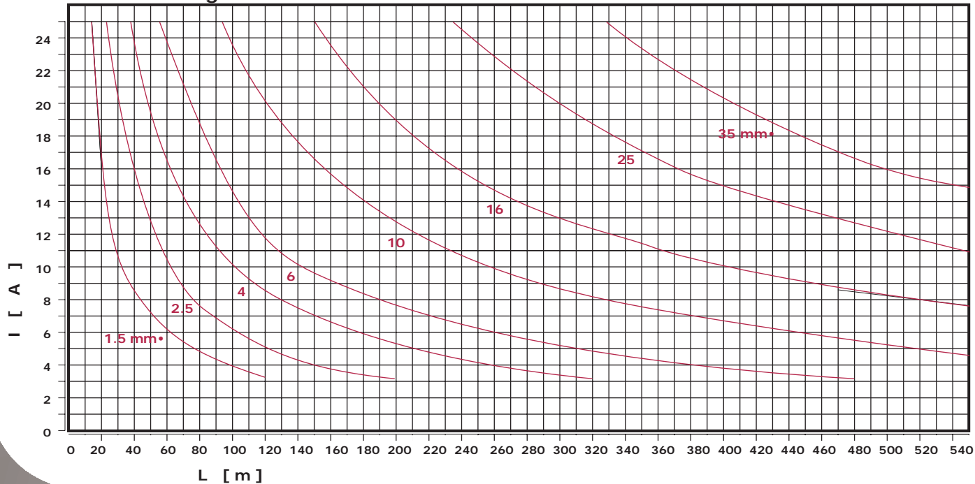
D.O.L. starting 230V multi-core cable
