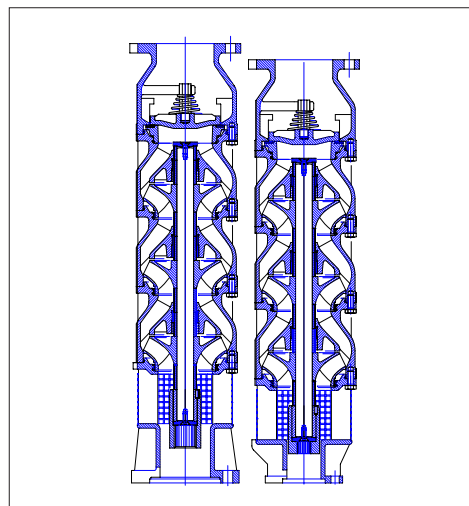
SECTIONAL VIEW
